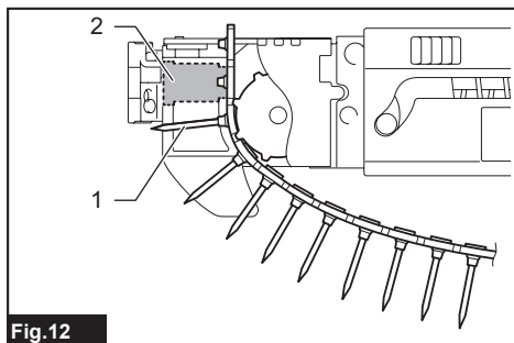
Fig.12 ▶ 1. First screw 2. Driving position
