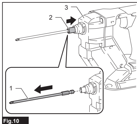
Fig.10 ▶ 1. Driver bit 2. Spindle 3. Gear housing
