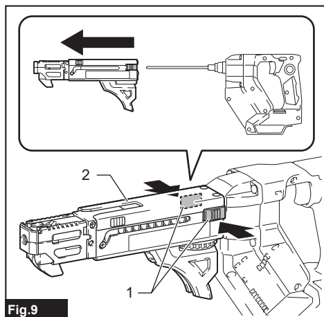
Fig.9 ▶ 1. Release buttons 2. Casing
