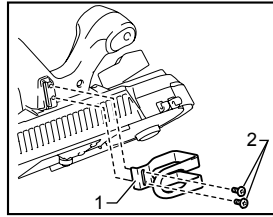
1. Hook 2. Screws
